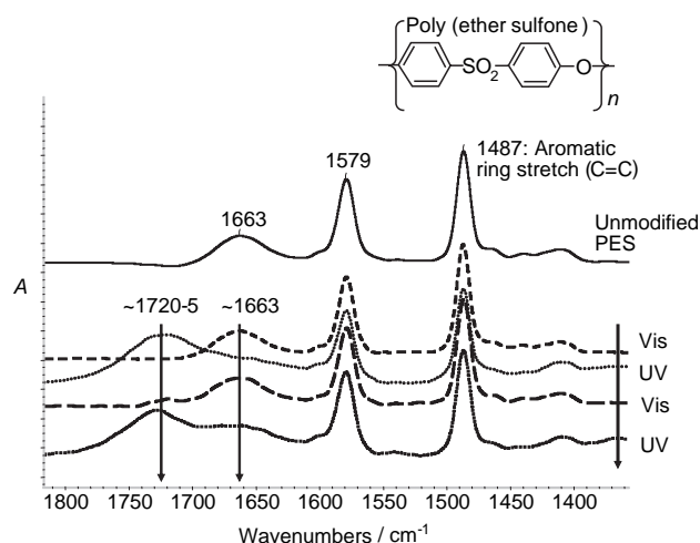
Figure 3. Five ATR/FTIR spectra of the unmodified (as received) PES ultrafiltration membrane and the spiropyran-grafted PES membrane after two cycles of exposure to UV irradiation at 254 nm for 1 h and visible light for 5 min. Note that the peak at \approx 1663 \text{ cm}^{-1} decreases whereas the peak at \approx 1720\text{--}1725 \text{ cm}^{-1} increases in intensity during exposure to UV at 254 nm.
