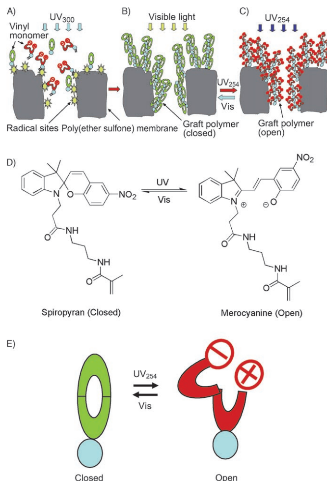
Figure 1. Schematic of graft polymerization and switching: A) Rensselaer's patented photografting process in which a synthetic ultrafiltration membrane formed from PES (photo sensitive polymer) is first dipped into a vinyl (spiropyran) monomer solution (1% w/v) in ethyl acetate for 1 h and then exposed to 300-nm UV irradiation to induce grafting and polymerization. B) Exposure of the grafted PES membrane to visible light for 1 h resulting in the formation of the "closed" apolar white form of spiropyran. C) Exposure of the grafted "closed" form of the PES membrane to UV irradiation at 254 nm for 1 h formed the "open" polar red form of spiropyran. D) The chemical structure of the vinyl spiropyran in two configurations as a function of UV and Vis irradiation. E) A schematic of the chemical structure of the vinyl spiropyran in two configurations as a function of UV and visible (Vis) irradiation.
