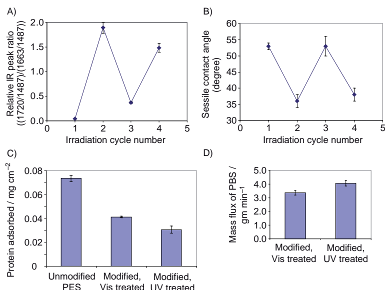
Figure 4. Summary data demonstrating the optically reversible switching of the wettability of the spiropyran grafted PES membrane surface after exposure to 254-nm UV light and visible light. A) Ratio of peak heights, R = (h_{1720}/h_{1487})/(h_{1663}/h_{1487}) , from ATR/FTIR spectra from Figure 3 as a function of alternating exposure to 254-nm UV light (1 h) and visible light (5 min) or cycle number. B) Surface wettability changes as measured by the sessile contact angle of the grafted PES membrane with a water droplet after alternating exposure to 254-nm UV light (1 h) and visible light (5 min) or cycle number. C) Adsorption of BSA in PBS (10 mM; pH 7.4) at 22 \pm 1^\circ\text{C} for 1 h on the as-received PES membrane and on modified PES membranes with grafted vinyl spiropyran in the “closed” (visible light) and “open” (254-nm UV light) configuration. D) Mass flux of PBS at pH 7.4 and 22 \pm 1^\circ\text{C} permeating through modified PES membranes with grafted vinyl spiropyran in the “closed” (visible light) and “open” (254-nm UV light) configuration after exposure to BSA adsorption from (C).
