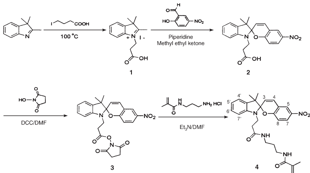
Scheme 1. Synthesis of the spiropyran-containing monomer compound 4 . DCC = dicyclohexyl carbodiimide.
